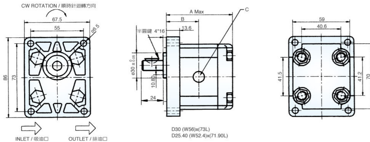
HGP-1A-F*-**-4BD-10 (DIN 4-bolt / 孔式)
